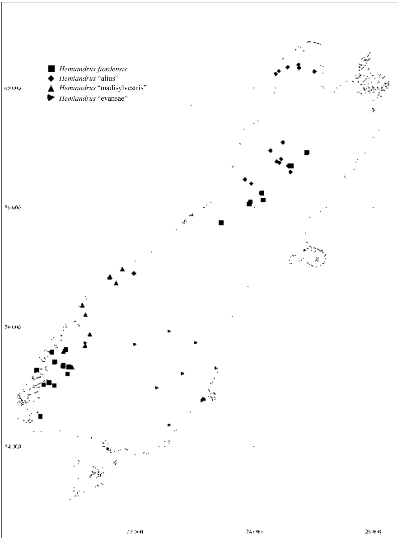
Figure 4. Distributions of Hemiandrus fiordensis , Hemiandrus "alius" , Hemiandrus "madisylvestris" , Hemiandrus "evansae" .
