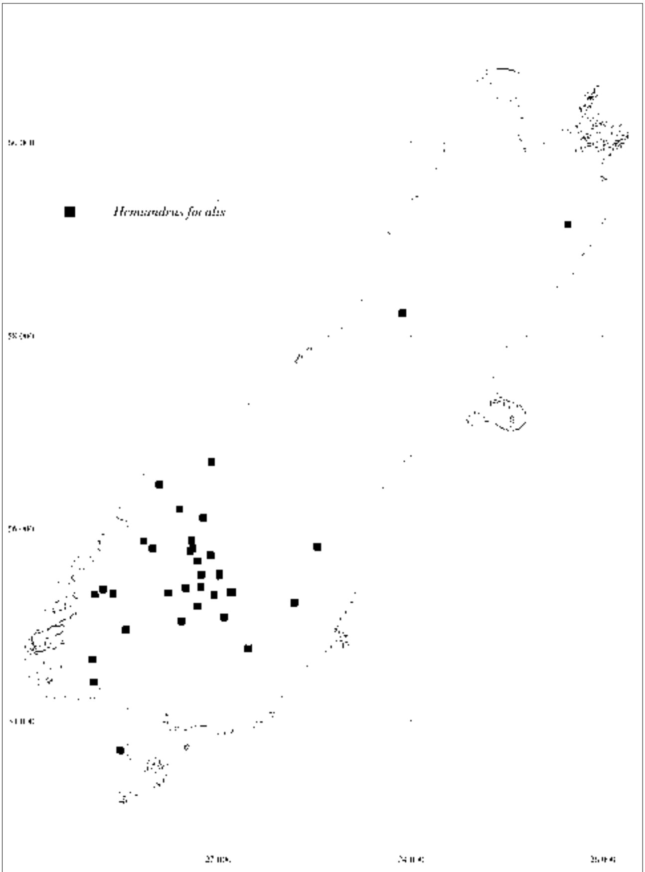
Figure 5. Distribution of Hemiandrus focalis .
