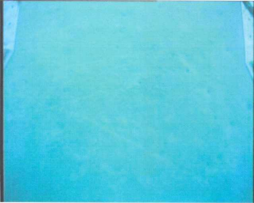
Site 1 A - Flat mud with hermit crab tracks
