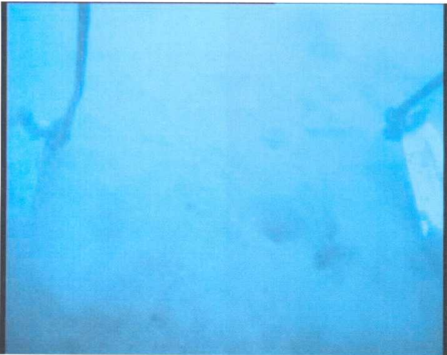
Site M1B - Mud bottom with burrows
