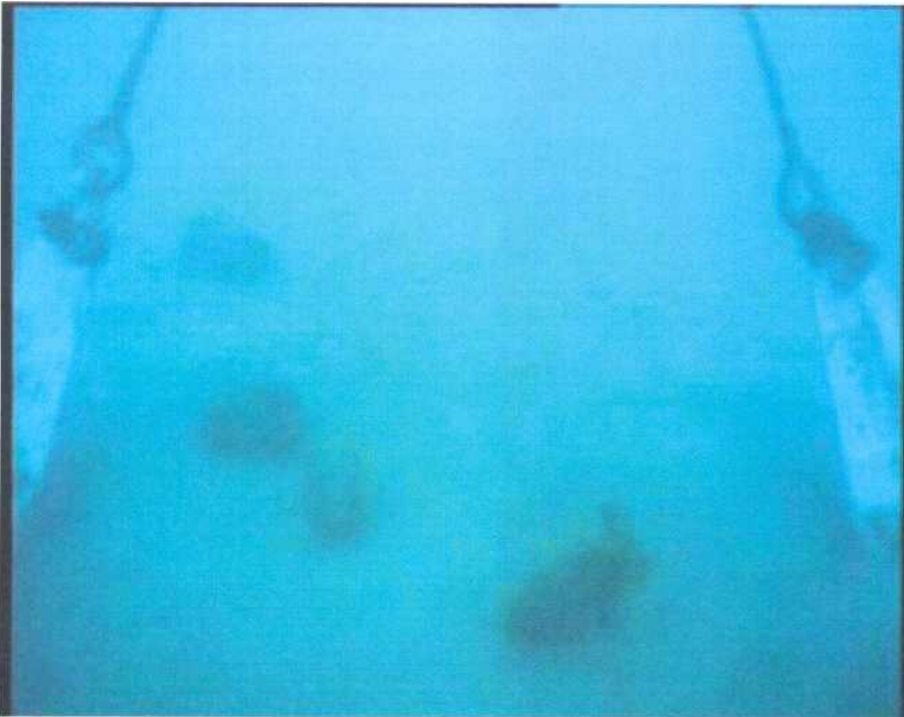
Site 1B - Horse mussels
