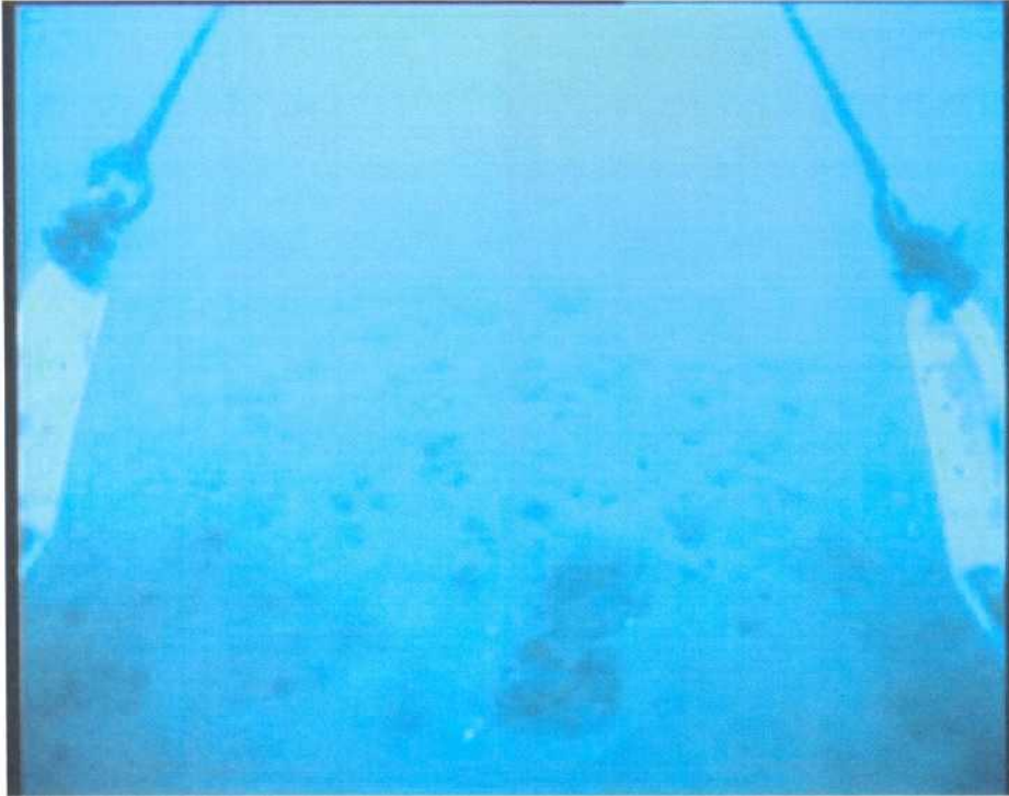
Site 5A - Mud with large burrow complexes
