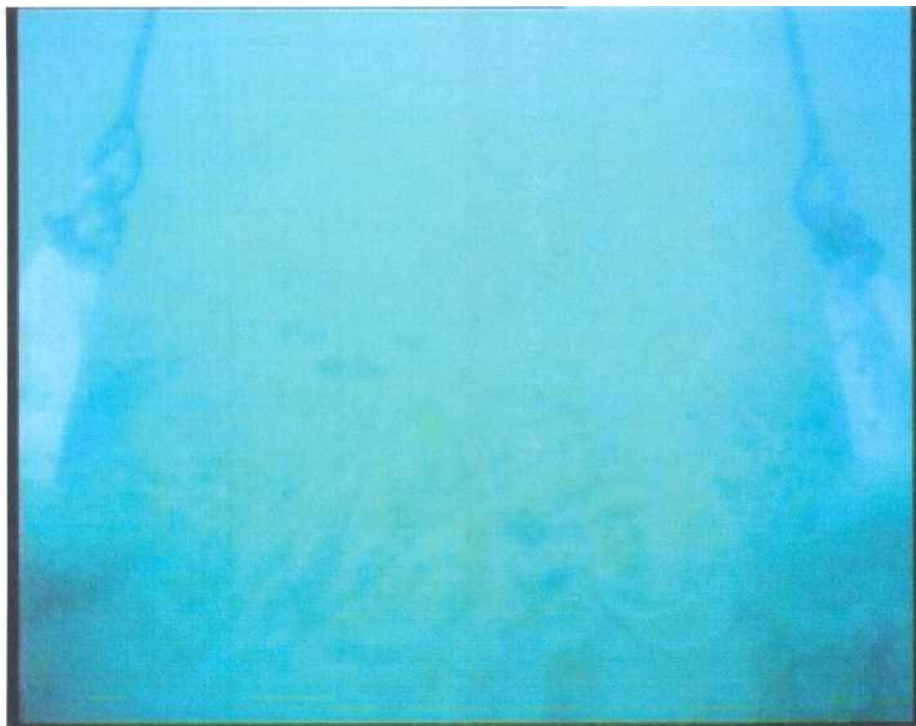
5C - Bottom with tracks
