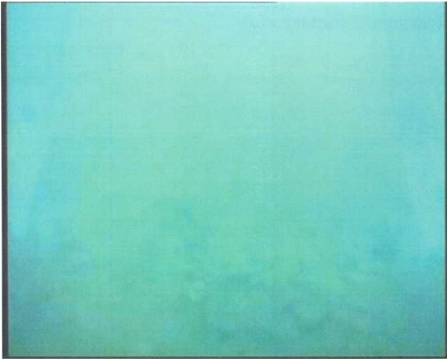
Site 2D - Dead dog cockle mounds
