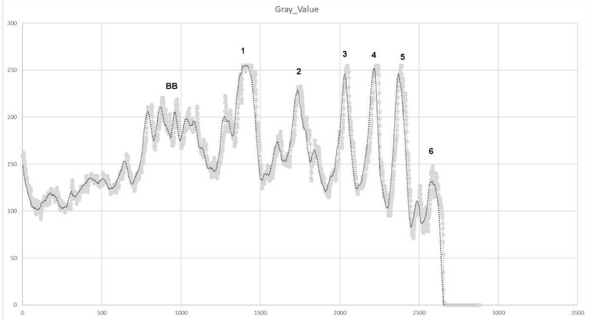
Thin section x-ray of ururoa_16 and its density profile (taken along the white line) indicating the number of band patterns. BB = birth band.
